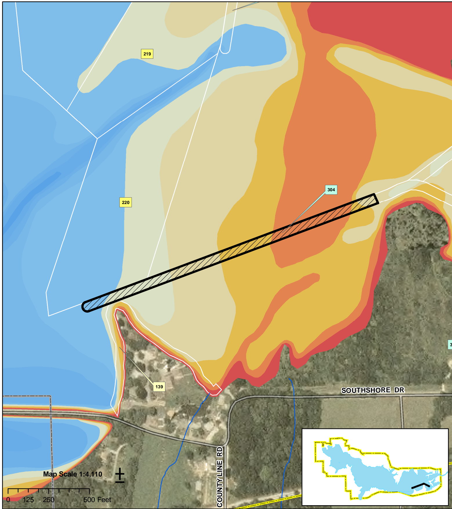
Lake Lemon SRP Map Showing Sediment Removal Area 304
